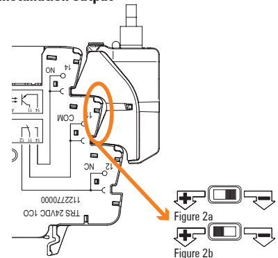
Figure 2a: Positive-switching logic: Potential change-over switch to "+", installation on output (11/14).
