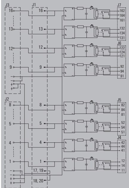
RSM-16 24 V AC/DC 1C0
