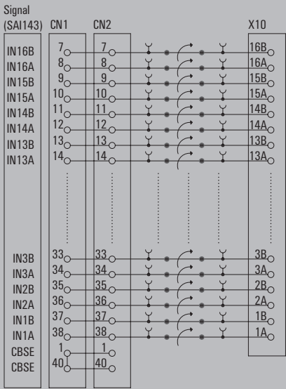
Connection for SAI143
