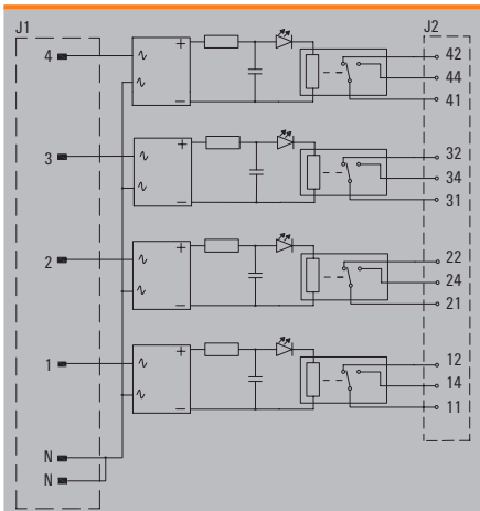
RSM-4 24 V AC/DC 1C0 RSM-4 115 V AC/DC 1C0
