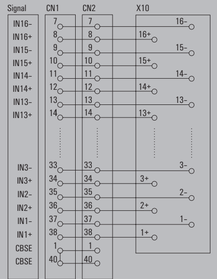
Schematic 1371180000/1371190000 (SAV144)
