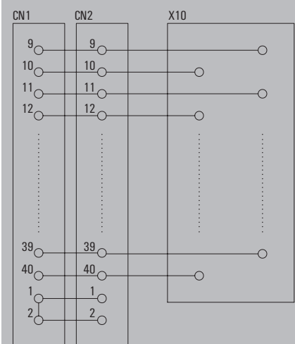
Schematic for 1371470000/1371500000
