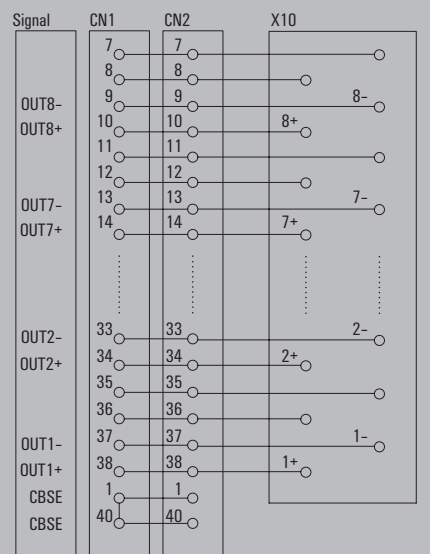
Schematic 1371200000/1371210000 (SAI533)
