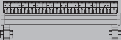
Field terminals view for SAI533
