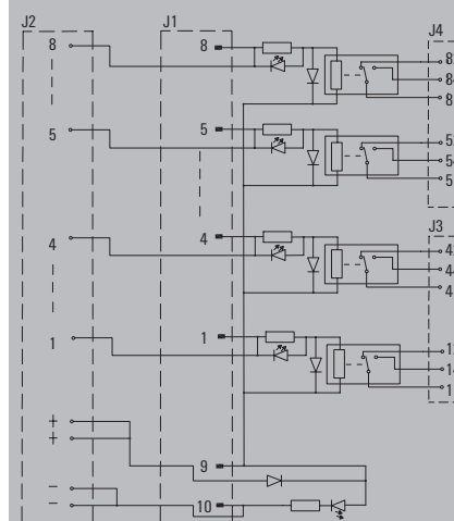
RSM-8 12 V-/24 V-/48 V- 1CO
