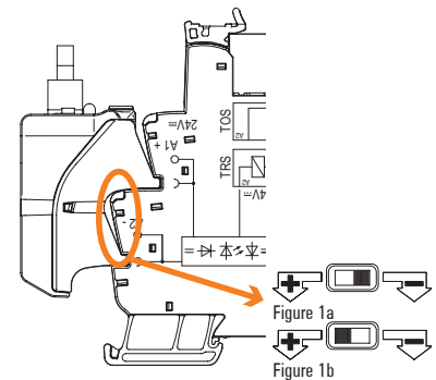
Figure 1a: Positive-switching logic: Potential change-over switch to "-", installation on 24 V DC input (A1/A2).
